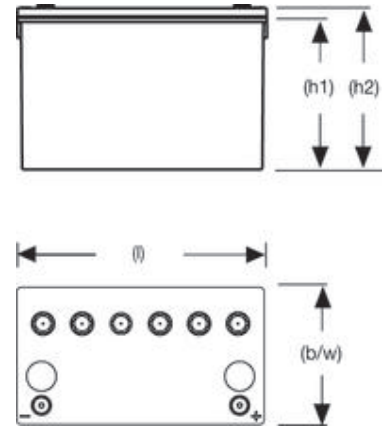
XL12V70
