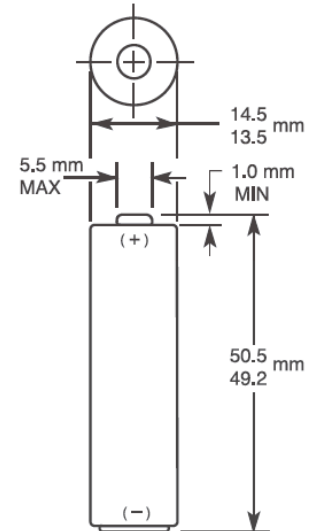
Dimensions shown are IEC standards
